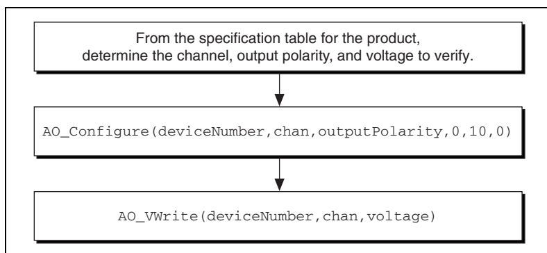
Figure 2. Analog Output Verification
